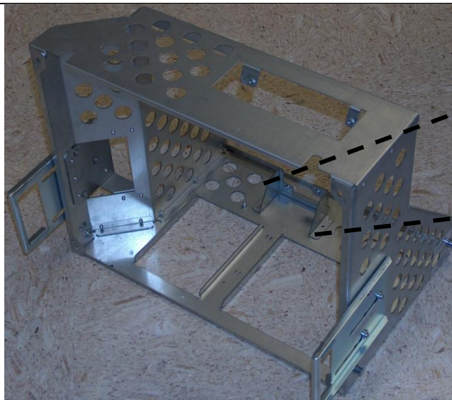
New Frame with bracket for larger plug
